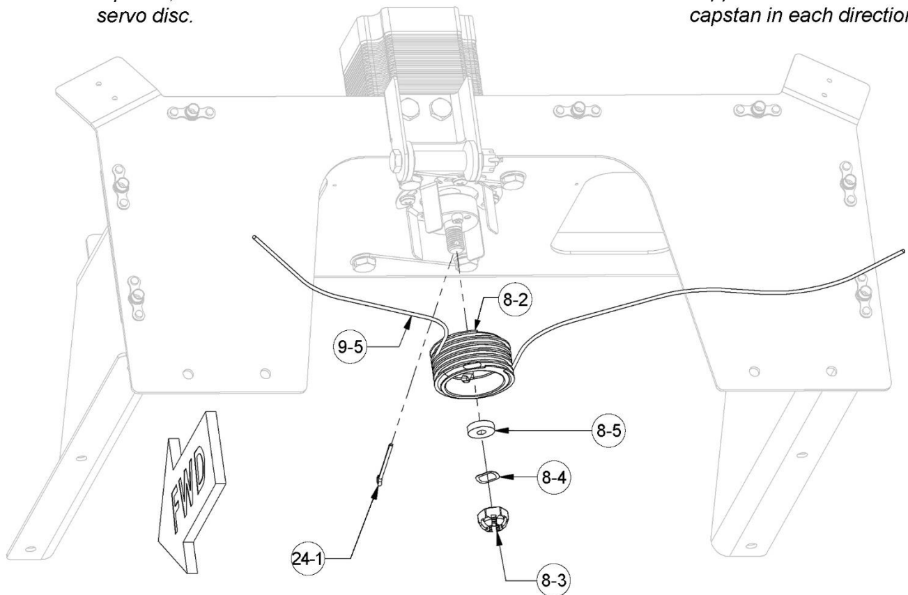
Figure 41: Installing Yaw Servo Capstan and Bridle Cable
