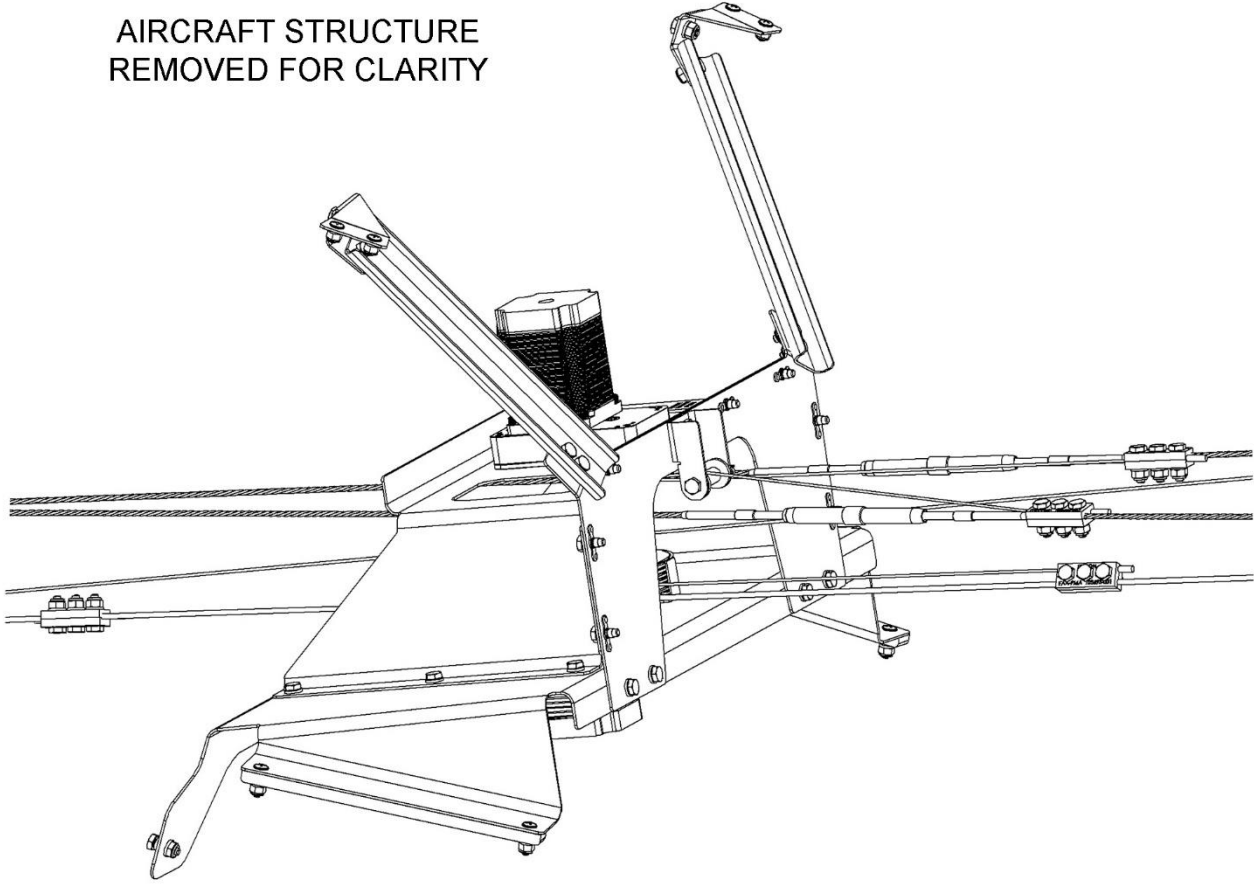
Figure 49: Pitch and Yaw Servos – Complete Installation
