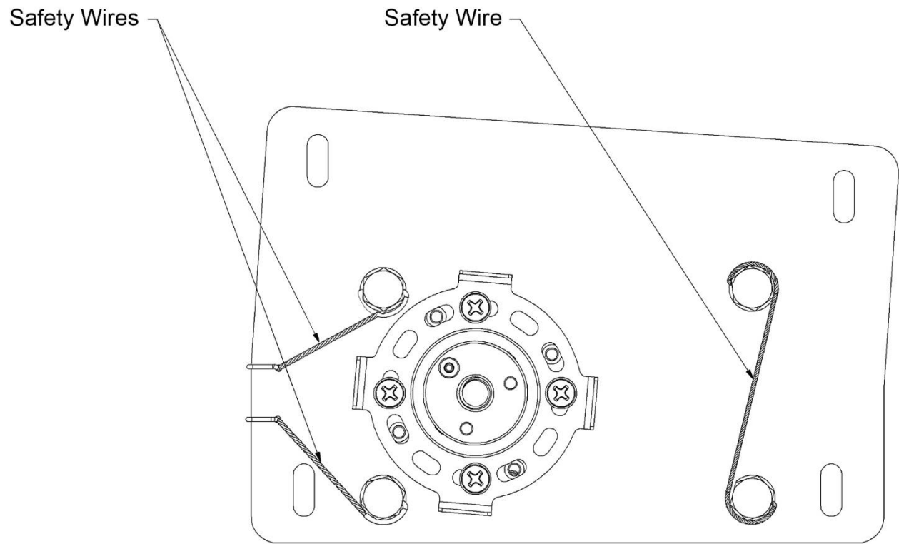
Figure 11: Safety Wiring Roll Servo Bolts (Example)
