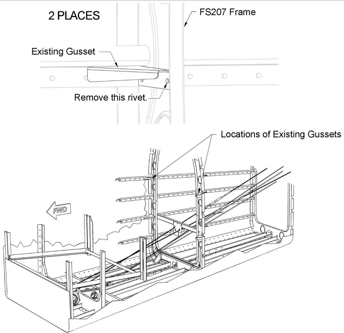
Figure 43: Removing Rivets on Existing Gussets
