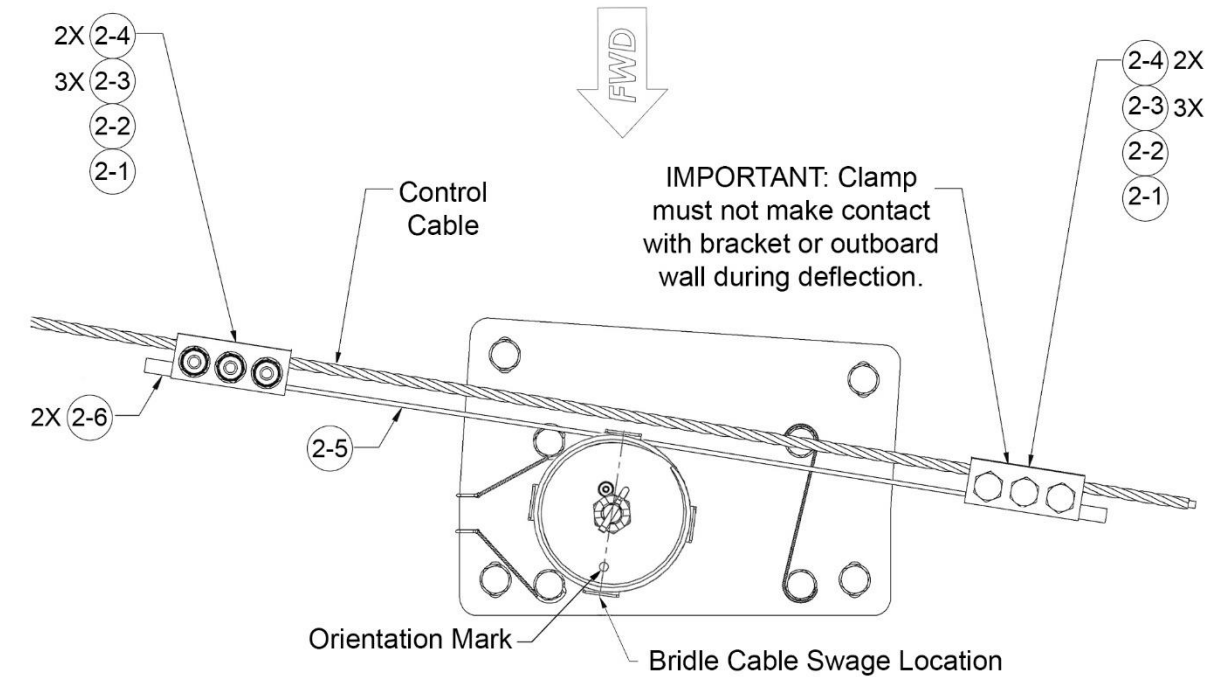
Figure 14: Installing Roll Servo Bridle Cable and Clamps – Outboard of Turnbuckle
