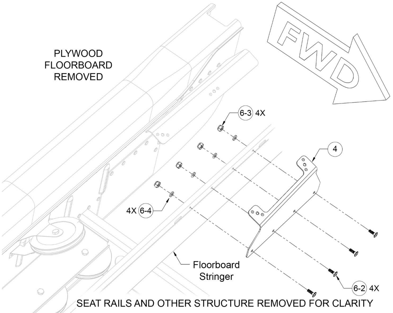
Figure 10: Securing Forward Support Bracket
