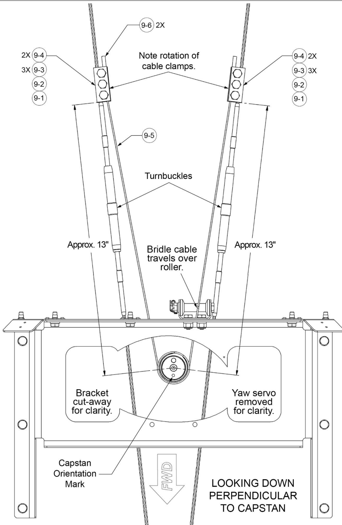
Figure 48: Connecting Yaw Servo Bridle Cable to Rudder Cable
