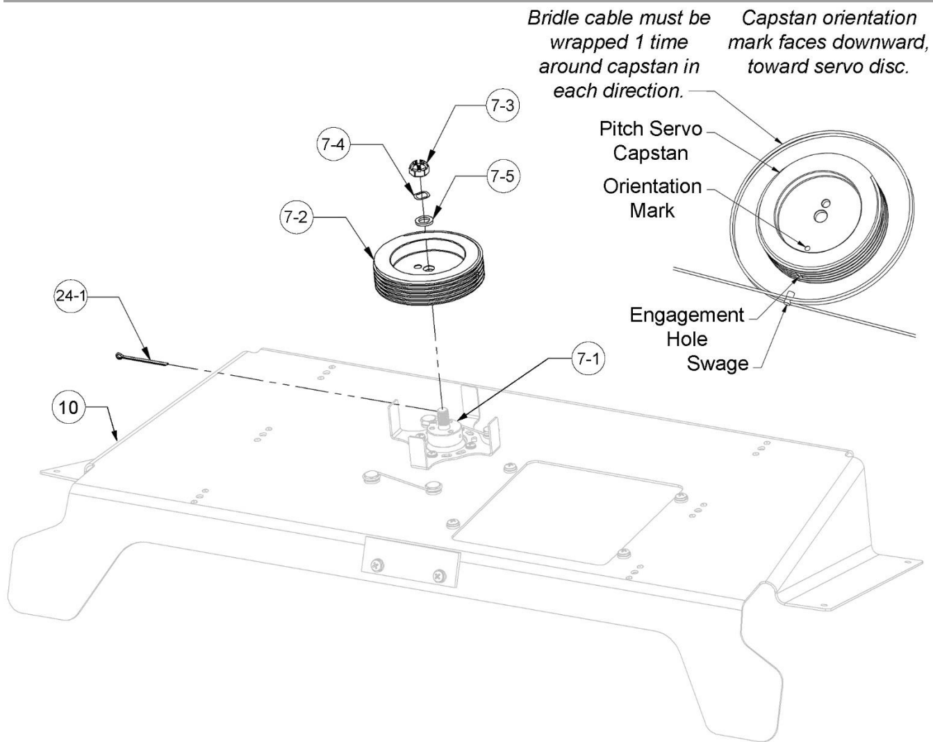
Figure 32: Installing Pitch Servo Capstan and Bridle Cable
