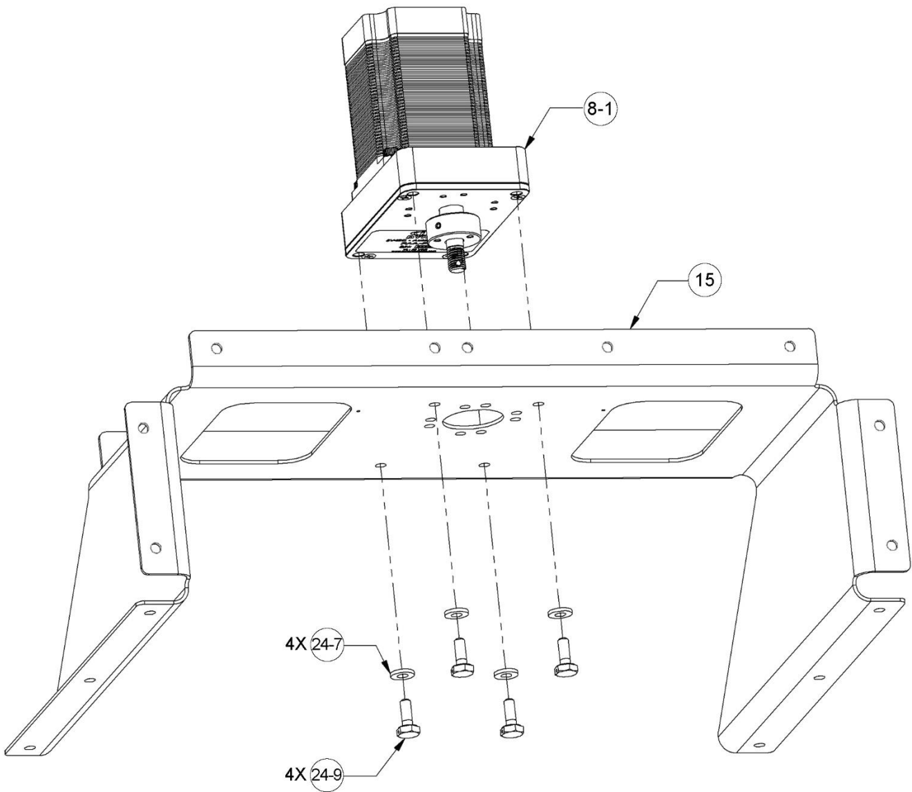
Figure 35: Attaching Yaw Servo to Bridge Bracket
