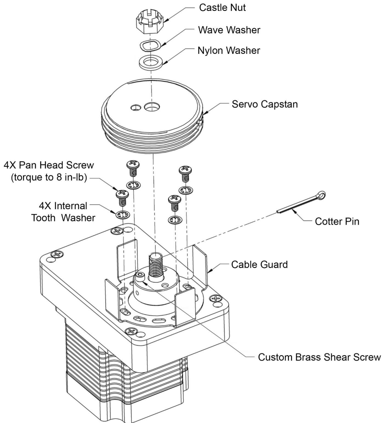
Figure 50: Exploded View of a Typical Servo Capstan Assembly
