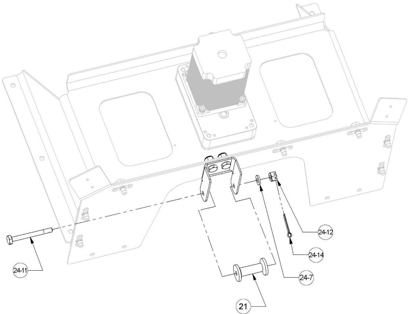
Figure 40: Installing Roller
