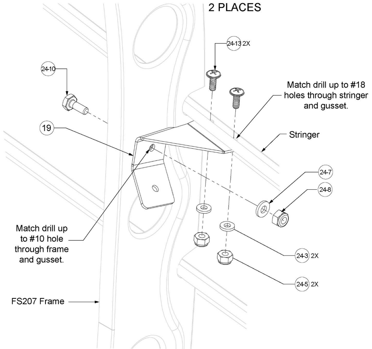
Figure 46: Attaching Gussets to Frame and Stringers (Right Side Shown)
