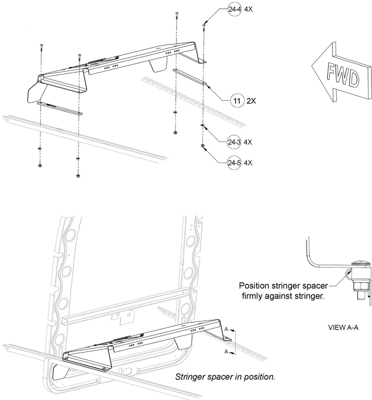
Figure 22: Positioning and Installing Shelf Bracket and Stringer Spacers
