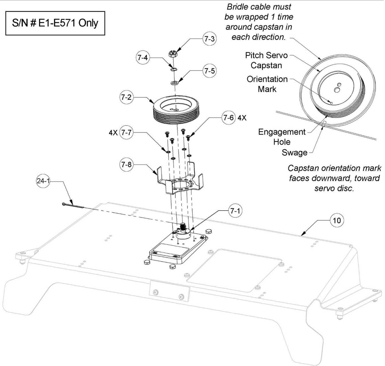
Figure 31: Installing Pitch Servo Capstan and Bridle Cable – S/N # E1-E571
