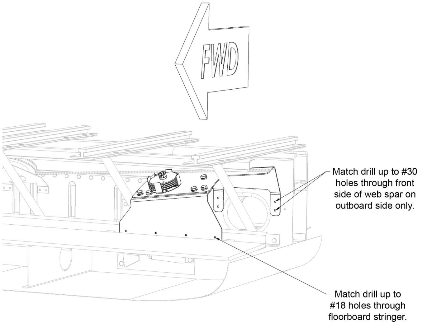
Figure 7: Drilling Holes for Roll Servo Brackets
