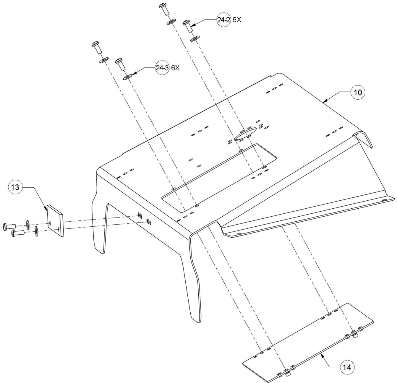
Figure 20: Attaching Cable Rub Strip and Optional Access Cover Plate
