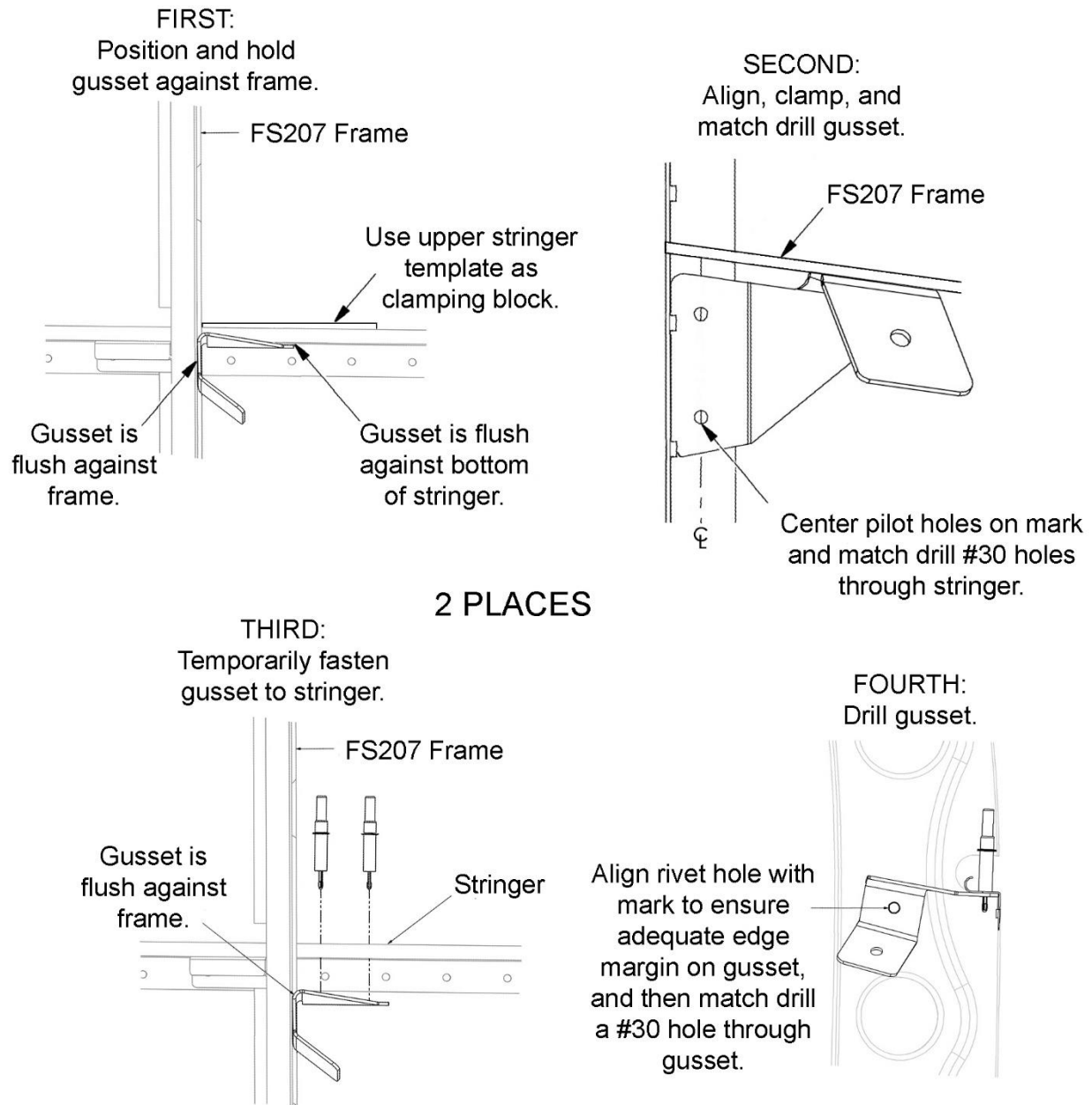
Figure 45: Temporarily Fastening Gussets to Stringers
