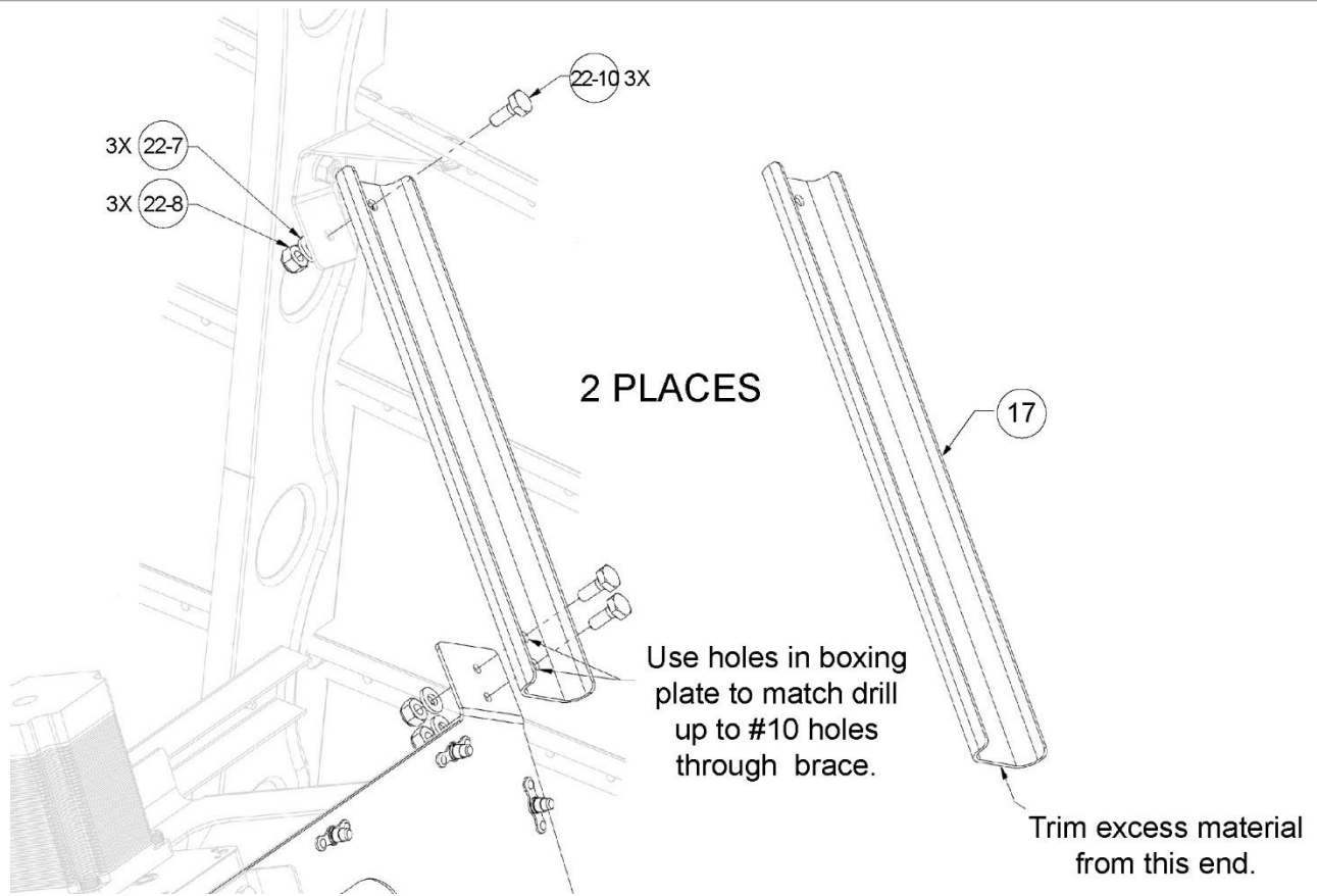
Figure 47: Attaching Bracket Assembly Braces (Right Side Shown)
