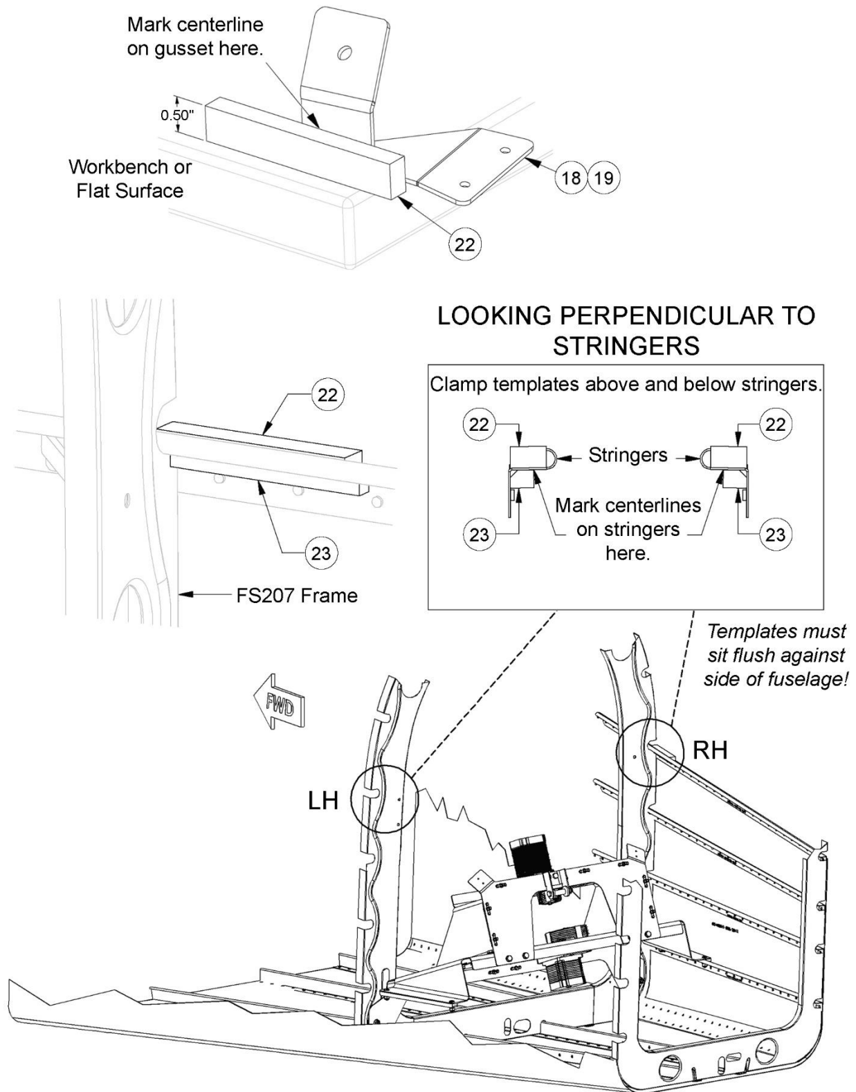
Figure 44: Marking Centerlines on Gussets and Stringers
