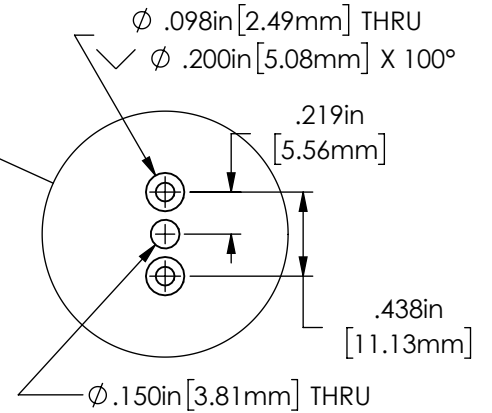
4 PLACES HOLE DETAIL FOR MK1000-06 NUTPLATE SCALE 1 : 1 (DO NOT SCALE DRAWING)
