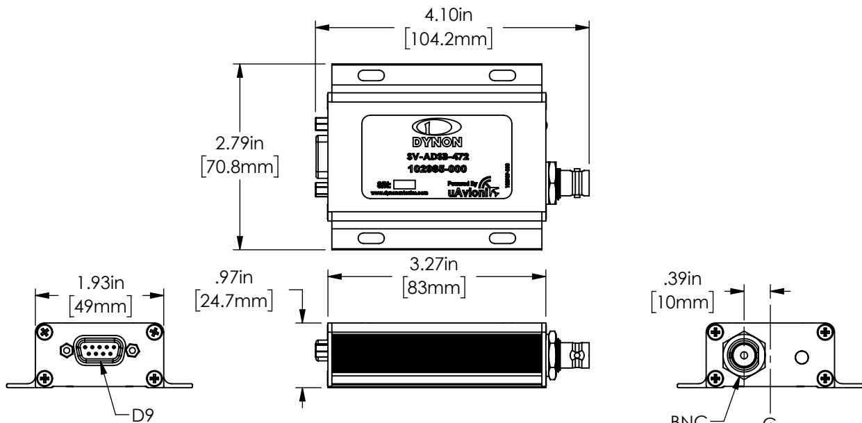
Physical Dimensions (SCALE 1:2)
